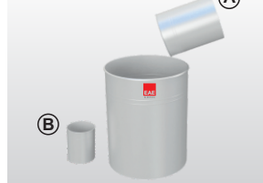
Resin and hardener are mixed in plastic bucket.
