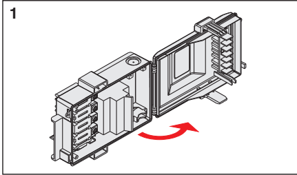
1- Open the cover of the plastic tap off box.
