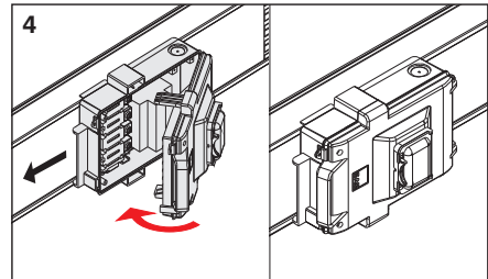
4- When the box is secured to the busbar housing, closed the box cover and tighten the screws.
