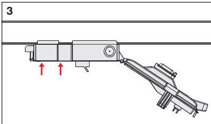
3- Carefully align the tap off box contacts and push the box towards the busbar.
