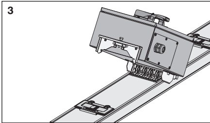
3- Carefully align the tap-off box contacts and push right side of tap-off box towards busbar and be sure fixing tap-off box firmly.
