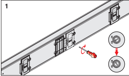
1- Open Plug-in cover by using screw driver.
