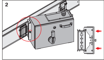
2- Release the plastic headed bolt to loosen mechanical fixing clamps. Push left side of tap-off box towards busbar and lock fixing clamps to the busbar. Tight back the plastic headed bolt to hold busbar rigidly.
