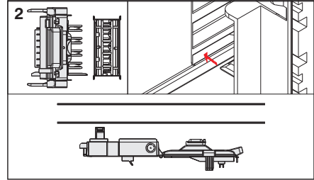
2- Hold the box in parallel to the busbar, check the position of the earth contact.
