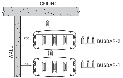
FIGURE 2 - EDGEWISE APPLICATION
