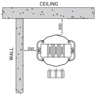
FIGURE 1 - EDGEWISE APPLICATION
