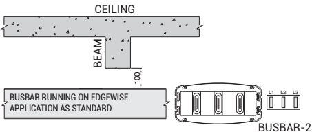
FIGURE 3 - CROSSING UNDER A BEAM ON EDGEWISE APPLICATION
