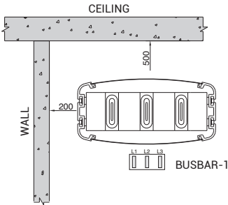
FIGURE 1 - EDGEWISE APPLICATION
