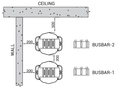
FIGURE 2 - EDGEWISE APPLICATION
