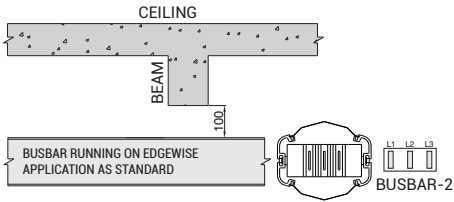
FIGURE 3 - CROSSING UNDER A BEAM ON EDGEWISE APPLICATION
